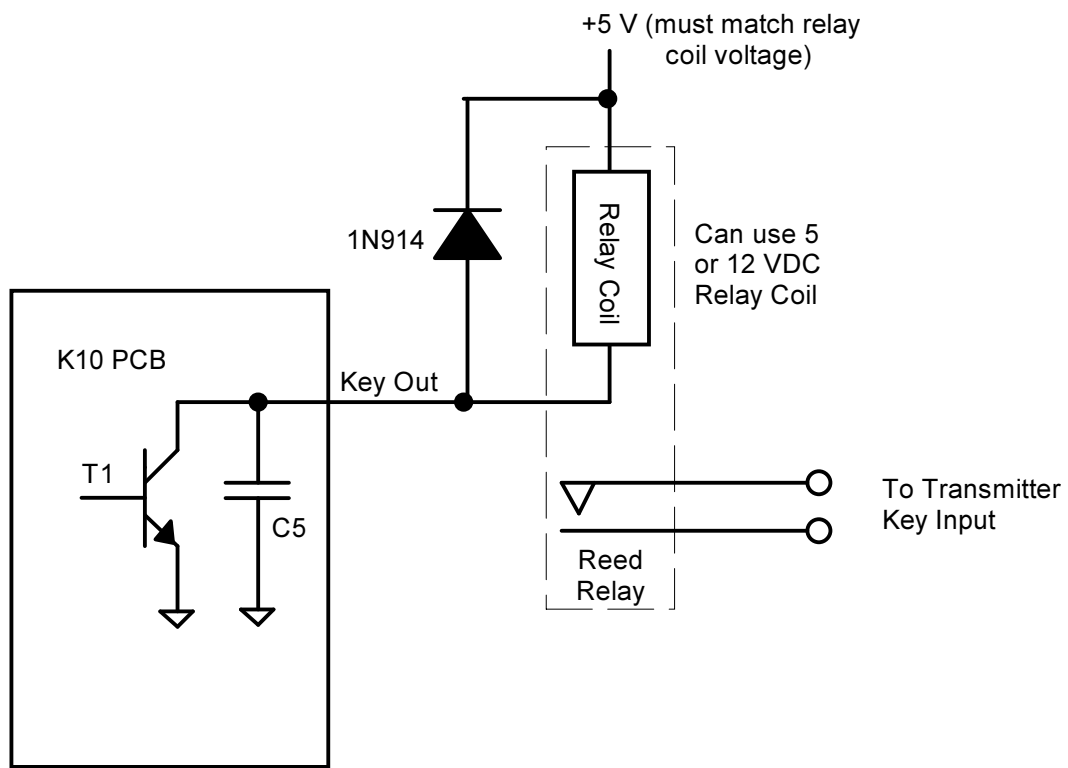
Schematic of Reed Relay Connection to K10 or K9 PCB
