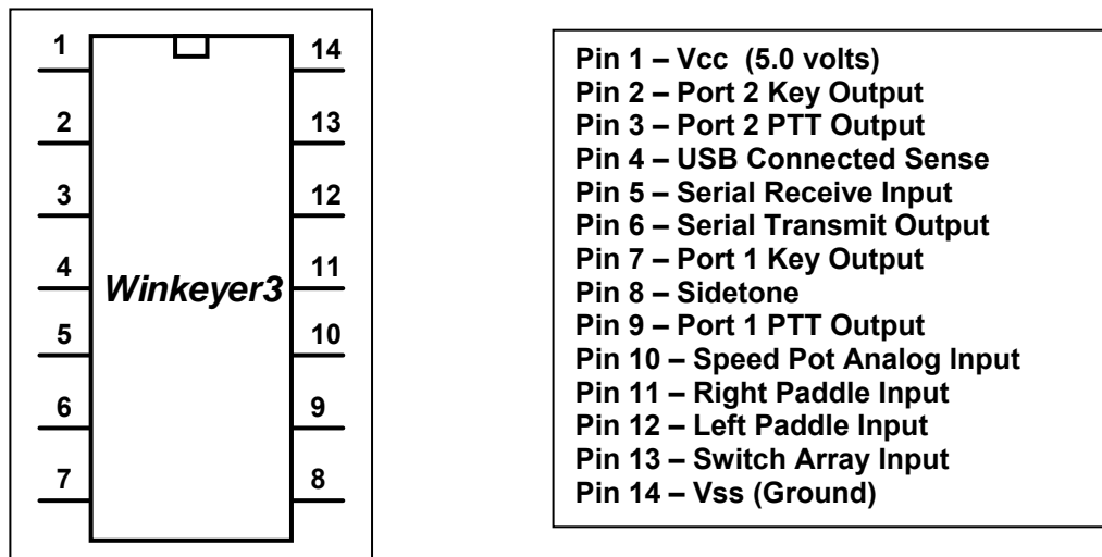
Figure 1 – Winkeyer3 Package & Pinout
